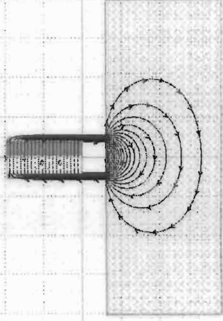
Magnet + Fe-weight + concentrator
