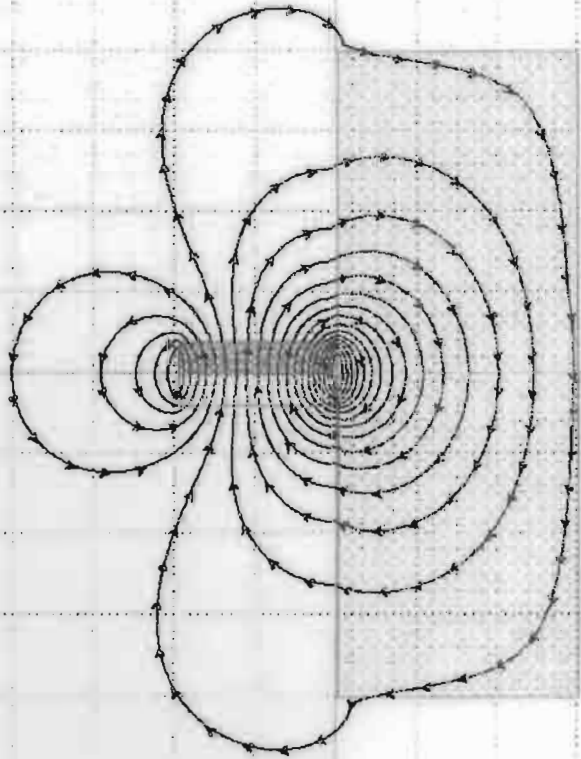
Magnet and Fe-weight
