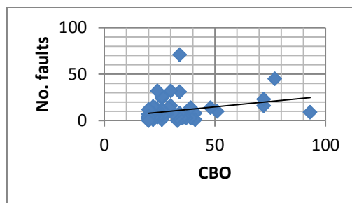
Figure 8: Eclipse JDT core, CBO vs faults – ‘ad-hoc coupled’ classes.
