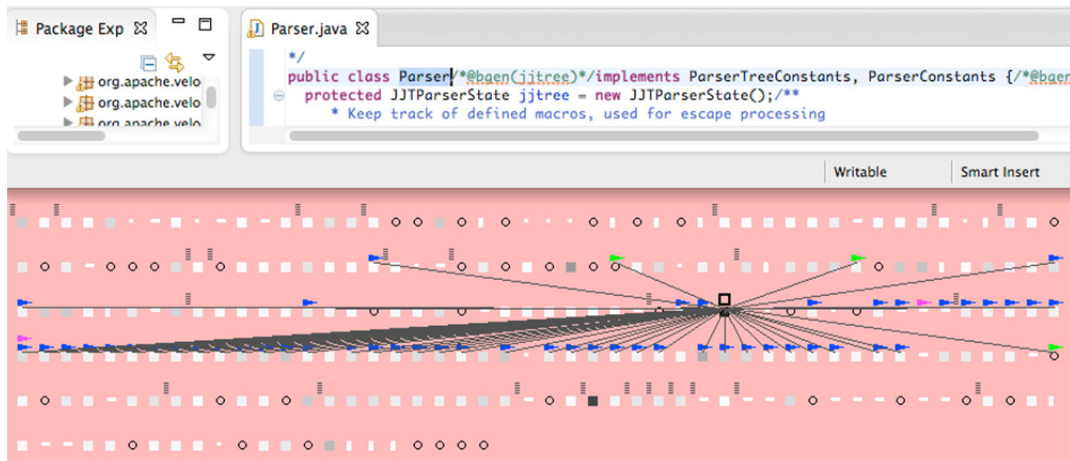
Figure 5: fan-out from Parser .
