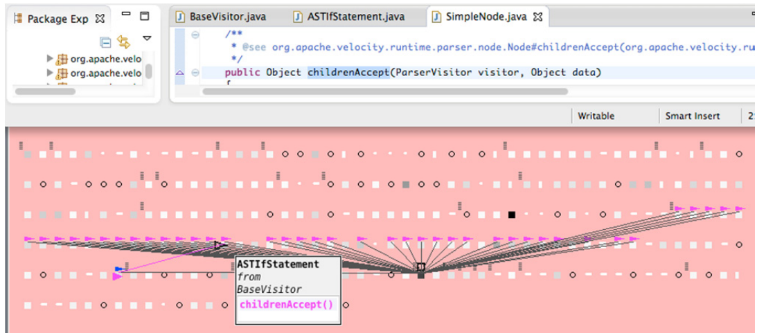
Figure 4: fan-out, foreign inheritance coupling BaseVisitor to ASTIfStatement .
