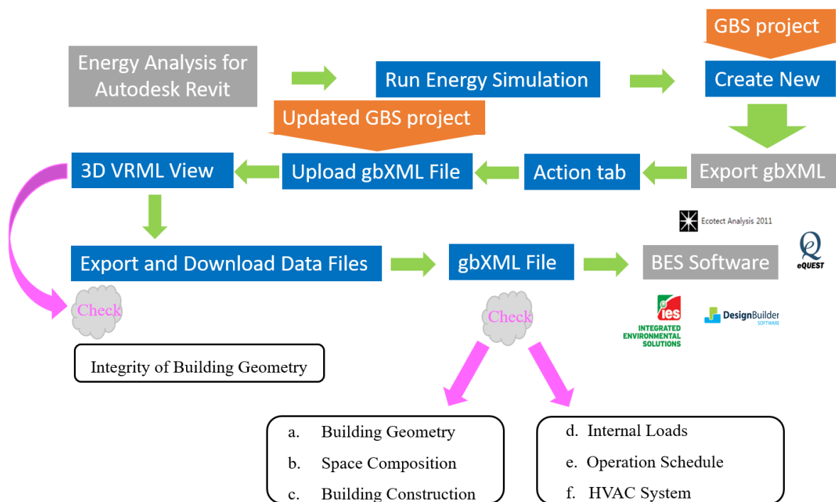
Figure 6: Process of creating gbXML file from Revit model
