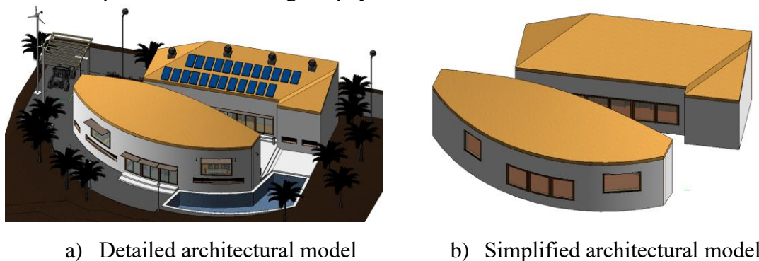
Figure 3: Model simplification
