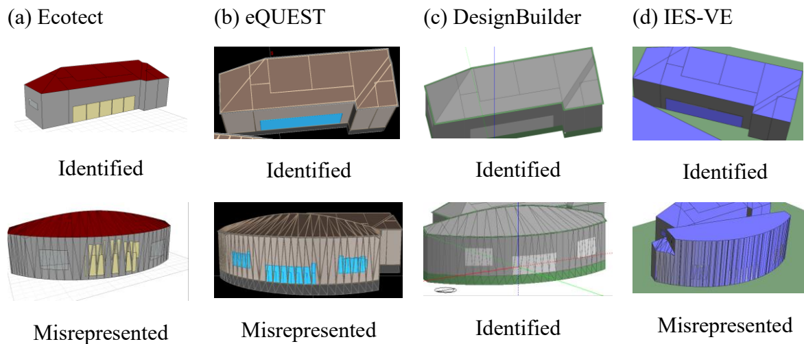
Figure 8: Building geometry of BIM model in BES tools: (a) Ecotect; (b) eQUEST; (c) DesignBuilder; (d) IES-VE
