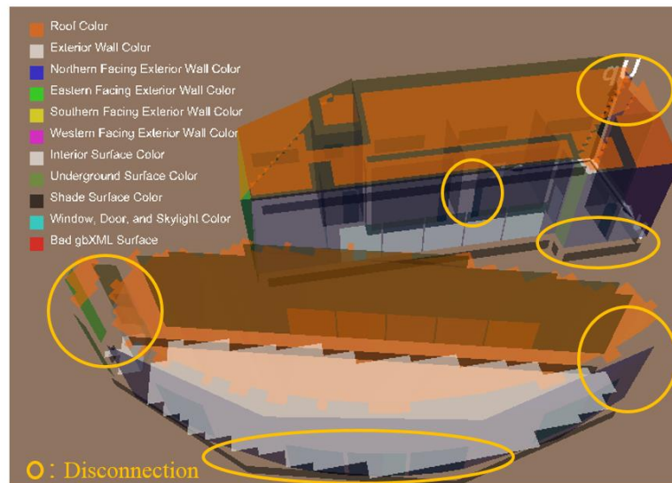
Figure 5: Disconnected building elements in 3D VRML view in GBS
