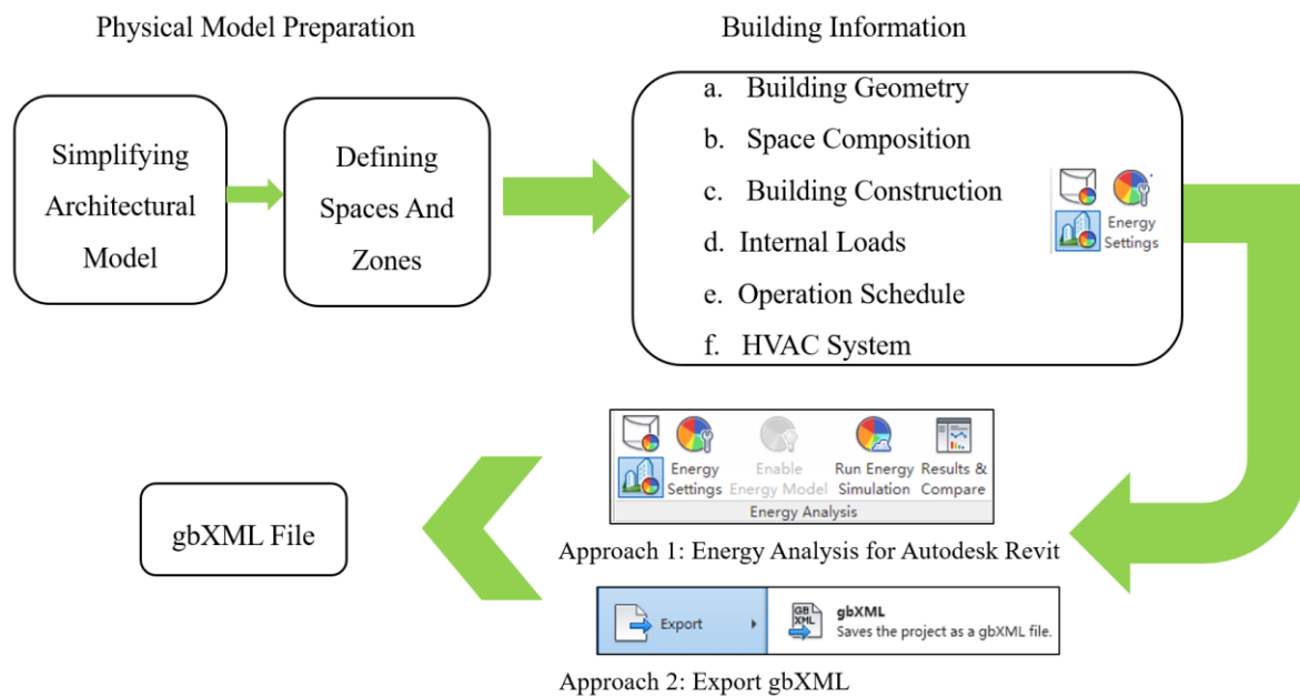
Figure 2: The process of exporting BIM-based information
