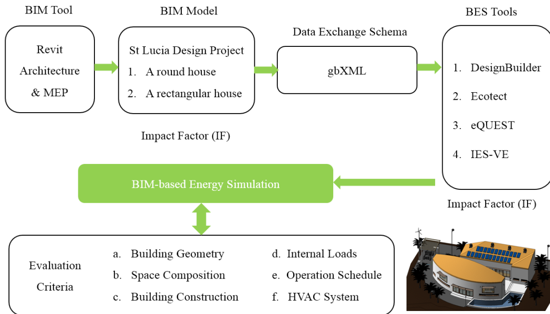
Figure 1: Workflow of interoperability investigation
