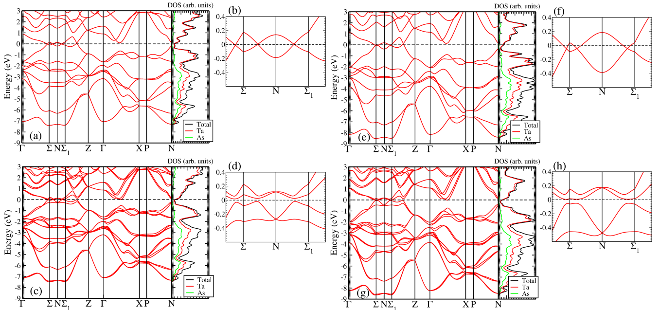
FIG. 6: (Color online) Electronic band structure of TaAs along the high-symmetry path through the Brillouin zone, calculated using PBEsol (a) and (b), PBEsol including spin-orbit coupling (SOC) (c) and (d), HSE06 (e) and (f), HSE06 including SOC (g) and (h). The Fermi energy is used as the reference. The zoom-ins (b) and (f) show the band crossings near the N point, which collapse to the Weyl points away from high symmetry paths in the BZ when SOC is included ((d) and (h)).
