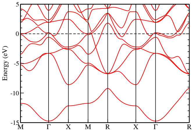
FIG. 3: (Color online) Energy band structure of TaAs in the CsCl phase (cubic Pm\bar{3}m ) at ambient pressure. The Fermi energy is used as the reference.
