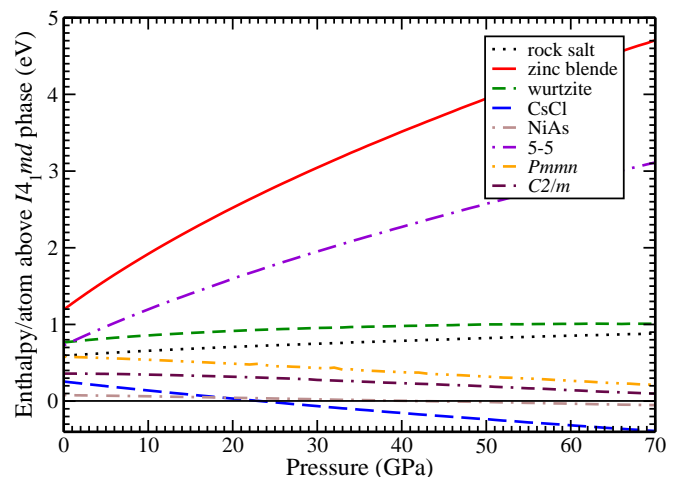
FIG. 2: (Color online) Enthalpy of each phase relative to that of the initial ground state phase ( I4_1md ), shown as a function of applied pressure. The phases studied are specified by their common names where available, otherwise the space group is given.
