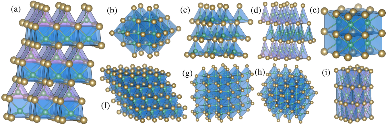
FIG. 1: (Color online) Crystal structure of the phases studied: (a) The ground state (body-centred tetragonal I4_1md ), (b) rock salt (cubic Fm\bar{3}m ), (c) zinc blende (cubic F\bar{4}3m ), (d) wurtzite (hexagonal P6_3mc ), (e) CsCl (cubic Pm\bar{3}m ), (f) NiAs (hexagonal P6_3/mmc ), (g) 5-5 (five-coordinated orthorhombic Cmc ), (h) six-coordinated orthorhombic ( Pmmn ), (i) monoclinic ( C2/m ) structure. The structures are shown as being built up of As-centred polyhedra (blue/purple (gray)), with As atoms in green (dark gray) and Ta atoms in gold (light gray).
