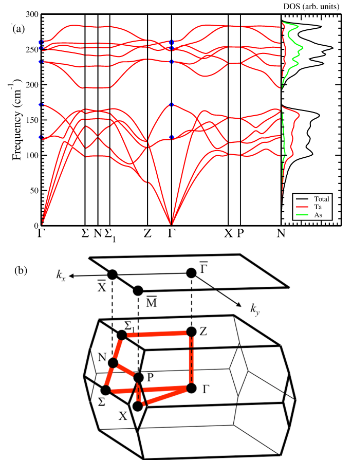
FIG. 5: (Color online) (a) Phonon dispersion and density of states (DOS), including projections onto the ion types in the unit cell, in the Brillouin zone. Inelastic Raman scattering measurements from Ref. 23 (blue diamonds) are included for comparison. (b) Schematic of the I4_1md bulk and (001) surface first Brillouin zones.
