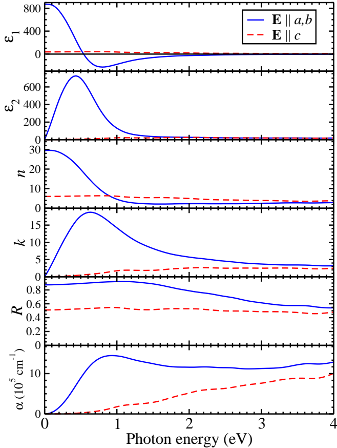
FIG. 4: (Color online) Dielectric function and derived optical parameters of TaAs as a function of photon energy: real ( \epsilon_1 ) and imaginary ( \epsilon_2 ) parts of the dielectric function, real ( n ) and imaginary ( k ) parts of the complex refractive index, reflectance R and absorption coefficient \alpha . The cases where the impinging electric field \mathbf{E} is parallel to the a or b directions (solid blue line) and parallel to c (red dashed line) are shown.
