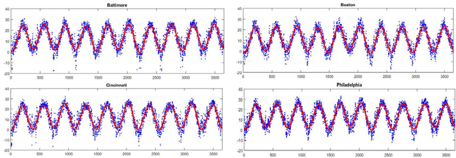
Fig. 2 DATs of Baltimore, Boston, Cincinnati and Philadelphia together with seasonal functions, from 1/1/1997 through 1/31/2006
