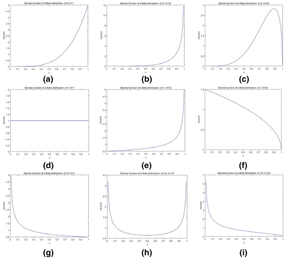
Fig. 1 Density functions of the Beta distribution B(a, b) with different values of the parameters: a = 1/2, 1, 5 ; b = 1/2, 1, 3/2
