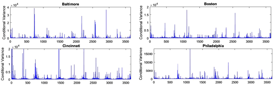
Fig. 4 Estimated conditional variance for each DAT series
