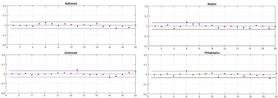
Fig. 3 Partial autocorrelation functions of the deseasonalized DAT time series
