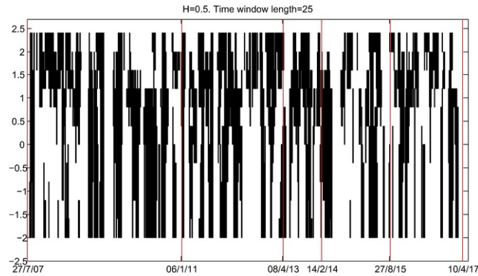
Fig. 12 Time-parameter plane. The black rectangles which left-bottom corner is given by (t, \beta_1) evidence the combination of parameter and time where the hypothesis of B_m of the mispricing calculated parameter \beta_1 cannot be rejected on time windows of length 25, starting at time t . The vertical lines point out the structural breaks.
