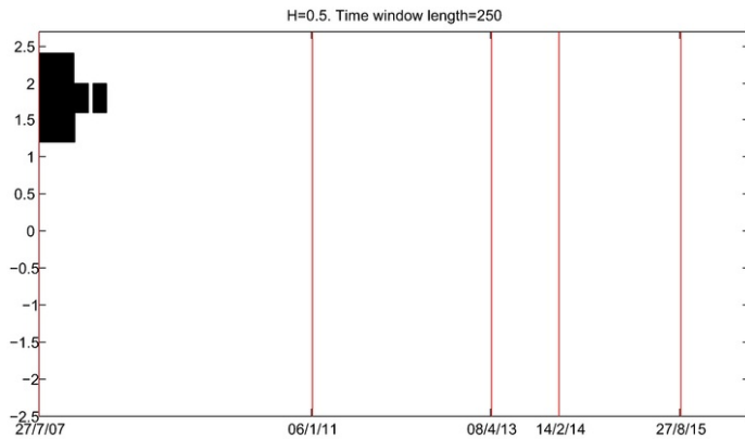
Fig. 21 Time-parameter plane. The black rectangles which left-bottom corner is given by (t, \beta_1) evidence the combination of parameter and time where the hypothesis of Bm of the mispricing calculated parameter \beta_1 cannot be rejected on time windows of length 250, starting at time t . The vertical lines point out the structural breaks.
