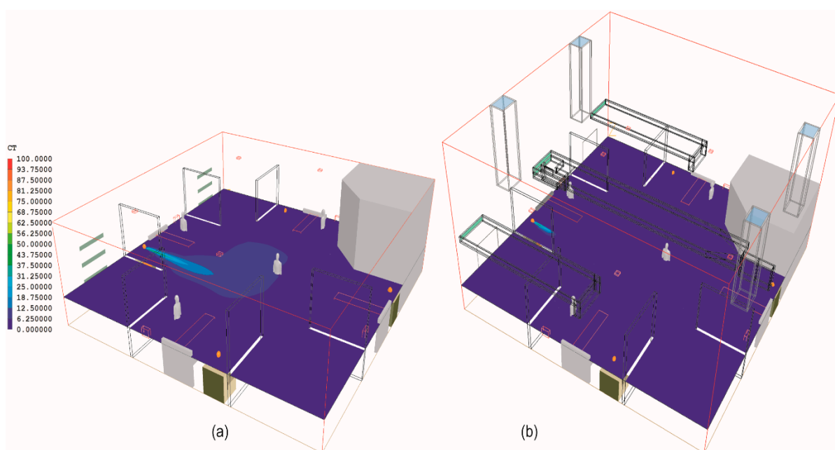
Figure 12. Differences in distribution of passive scalar airborne contaminants in Cruciform Ward based on: (a) Window design; (b) NPV system design.
