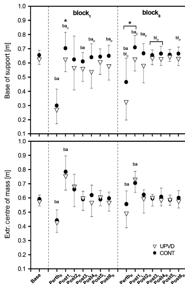
Figure 4. Base of support and extrapolated centre of mass at touchdown (TD) during nonperturbed walking (base: average values of 12 consecutive steps), at TD of the perturbed leg (pert R ), and at TD of the following six consecutive steps to an unexpected perturbation (post 1L –post 6R ) for unilateral peripheral vestibular disorder (UPVD; n = 13 ) patients and matched healthy controls (CONT; n = 13 ) during the first (block 1 ) and the final (block 8 ) unexpected perturbation during treadmill walking (set speed of 1.4 \text{ m}\cdot\text{s}^{-1} ; mean and SD). In order to maintain a stable body configuration (i.e., positive margin of stability) the base of support must exceed the extrapolated center of mass. Please note that for the base of support there were tendencies ( P < 0.1 ) for differences from baseline for the UPVD patients in block 1 for post 2R and post 5L . ba: Statistically significant difference to base for both subjects groups ( P < 0.05 ). ba p : Statistically significant difference to base for the UPVD group ( P < 0.05 ). bl: Statistically significant difference to block 1 for both subjects groups ( P < 0.05 ). bl c : Statistically significant difference to block 1 for the control group ( P < 0.05 ). bl p : Statistically significant difference to block 1 for the UPVD group ( P < 0.05 ). *Statistically significant difference between the UPVD and control groups ( P < 0.05 ).
