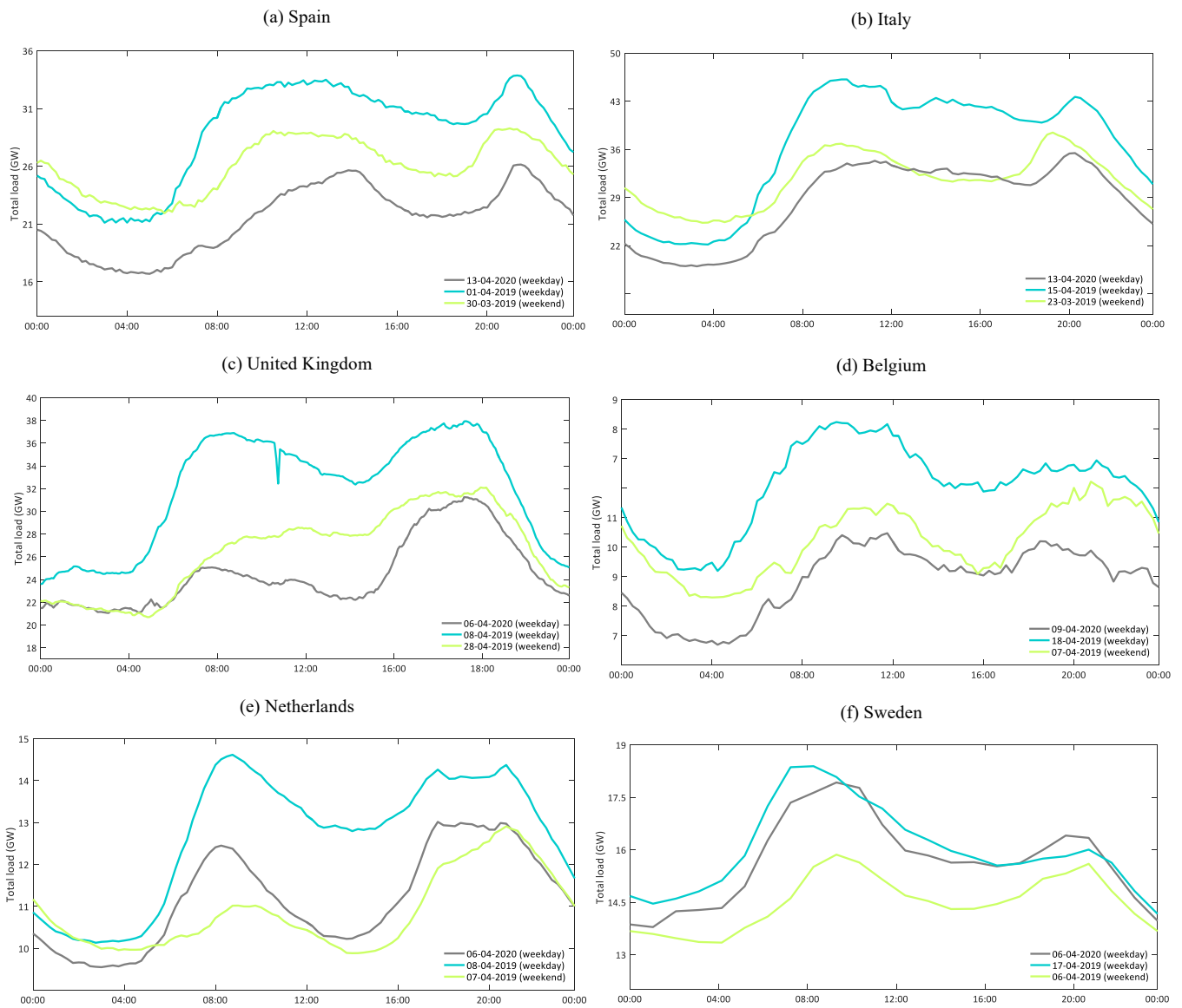
Fig. 3. Daily load profile comparison for a weekday of April 2020, a reference weekday and a weekend in 2019 for (a) Peninsular Spain [3], (b) Italy [4], (c) the UK [5], (d) Belgium [6], (e) Netherlands [7], and (f) Sweden [7]
